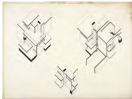
Residence for Mrs. MacBride Axonometric drawing Ann Arbor, Michigan, 1926 Gouache & pencil on paper 18 3/4 x 24 3/4 inches (47.6 x 62.9 cm) (KLH 61)
